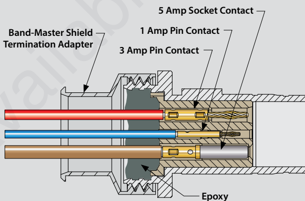
Series 880 QDC Plug
