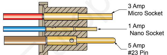
Unshrouded Type A Insert
