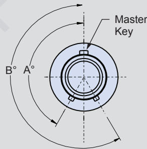
Plug Key Positions
